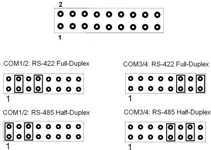
JP7 RS-232/422/485 Default Jumper Settings
