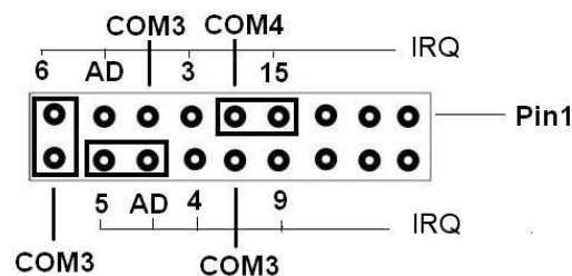
JP6 Jumper Block with Default Settings
