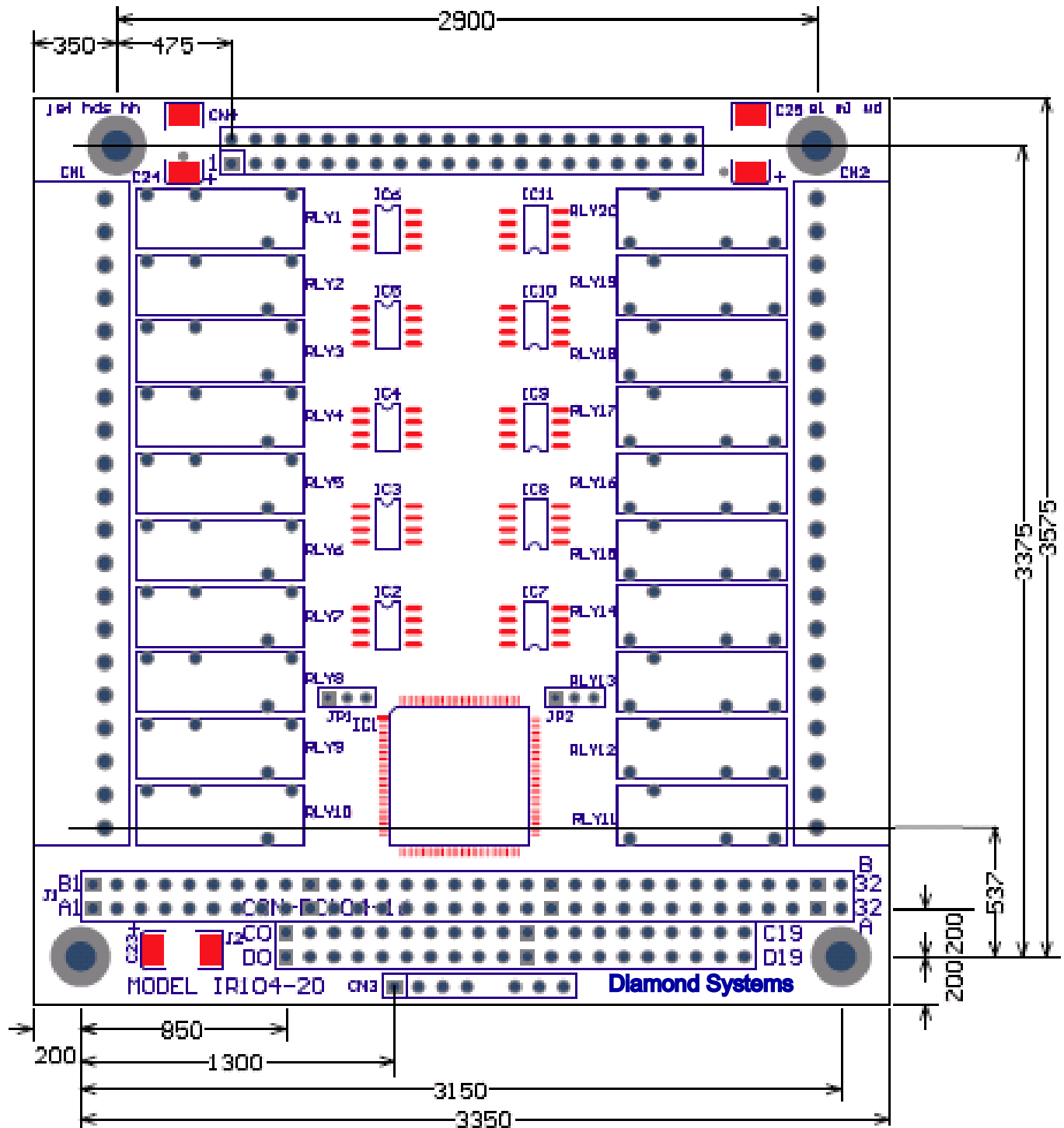
Mechanical Layout for IR104 All Dimensions in mils (1000 mils = 1 inch)
